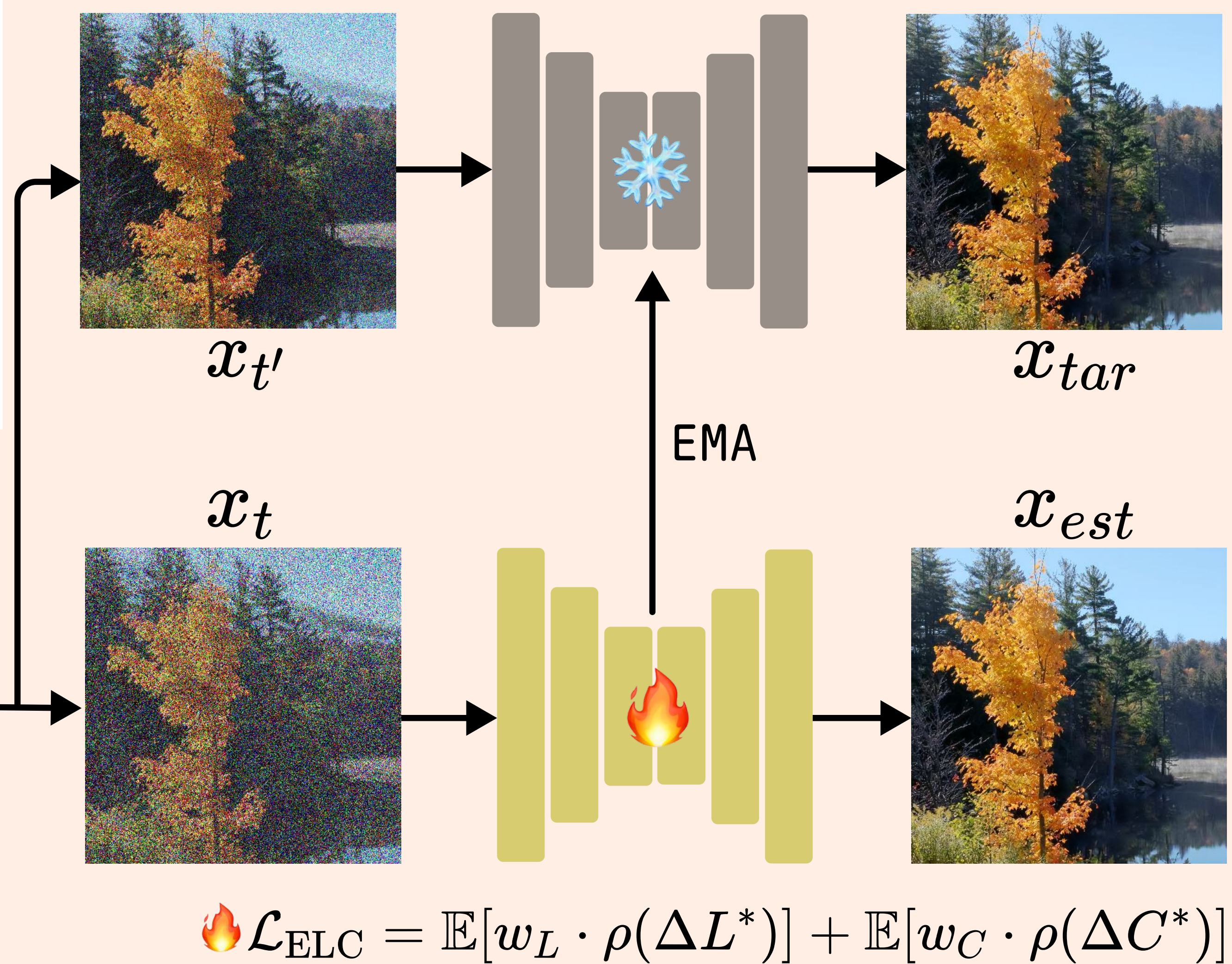
(c) Exposure-Aware Consistency Model
