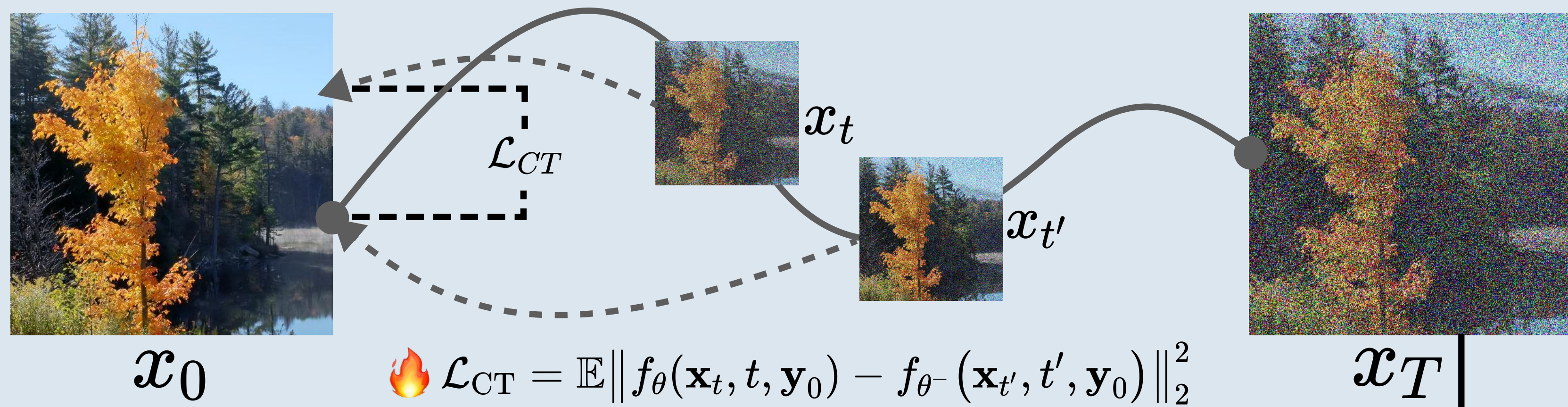
(a) Illustration of Consistency Training
